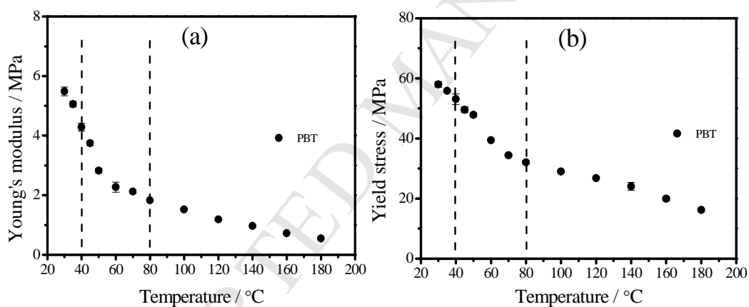
Young's modulus (a) and yield stress (b) of PBT at various temperatures.
