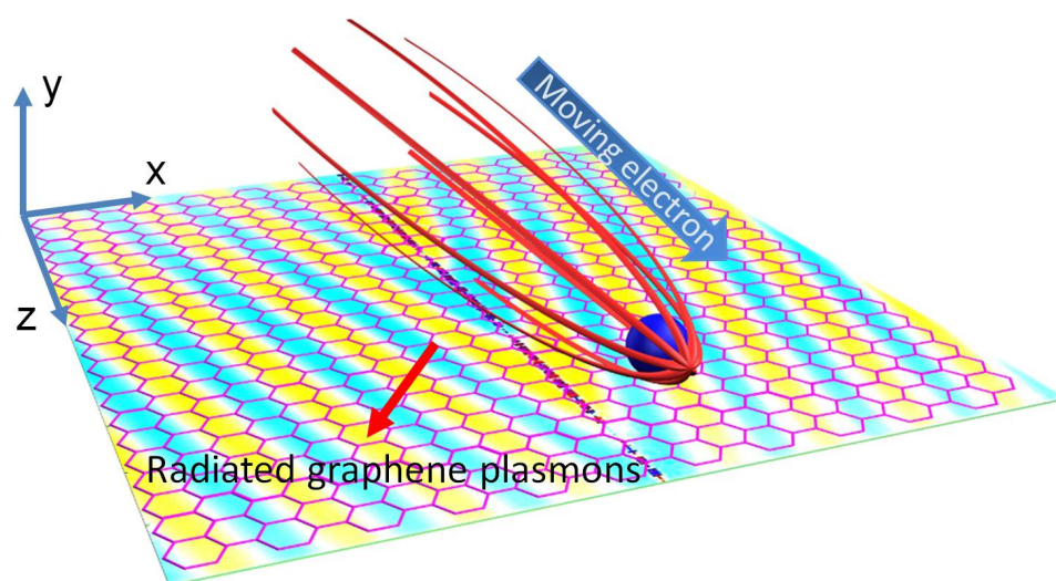
Schematic of an electron moving above a graphene layer along the z direction with a constant velocity v .
