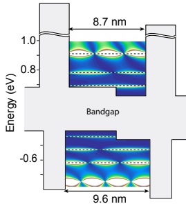
1D model LDOS
