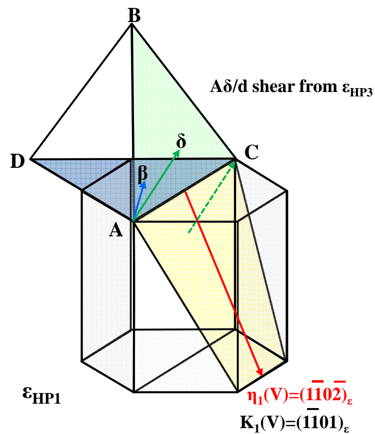
\{10\bar{1}1\} Twinning
