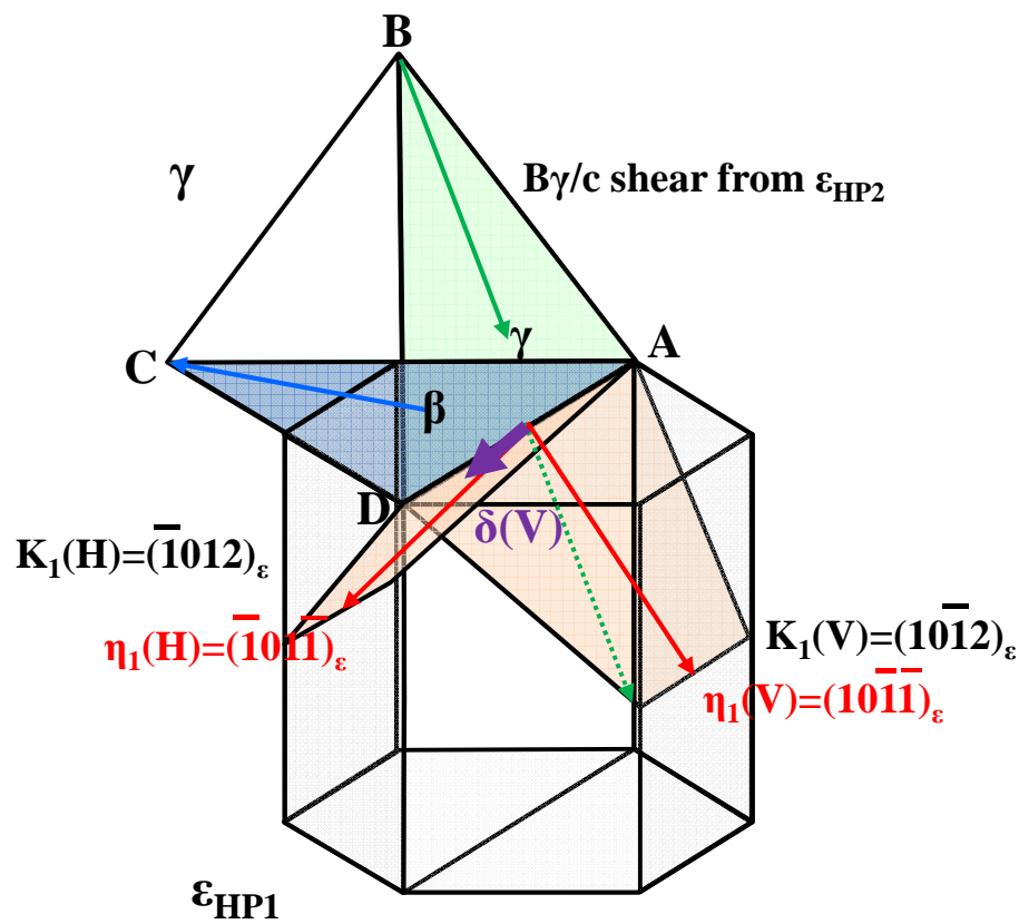
\{10\bar{1}2\} Twinning
