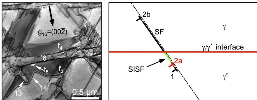
Nucleation of stacking fault in single crystal Ni-base superalloy
