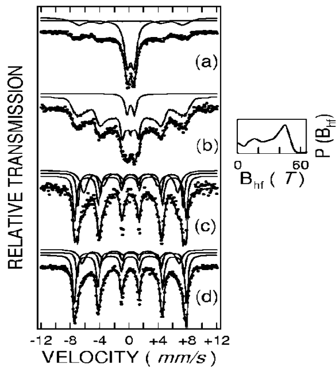
Fig. 1. Mössbauer spectra of \text{CoFe}_{1.6}\text{Cr}_{0.4}\text{O}_4 sample annealed at (a) 200 °C (b) 400 °C (c) 600 °C and (d) 800 °C.
