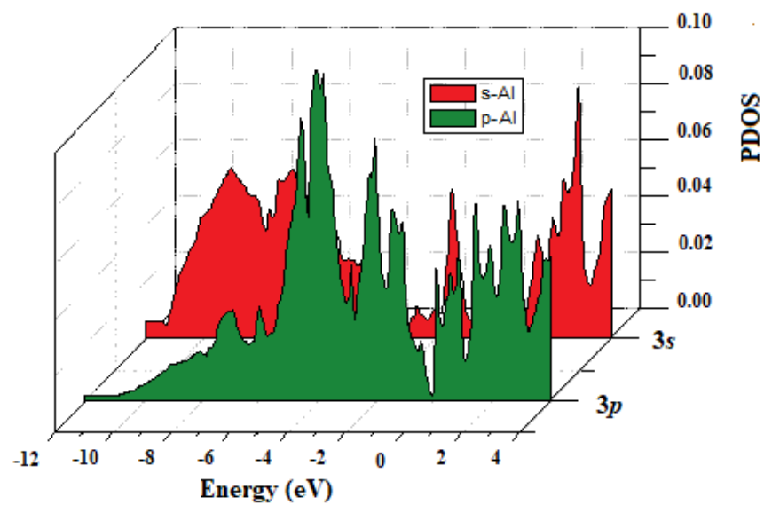
Figure. Partial DOS for 3s and 3p states of aluminum atom
