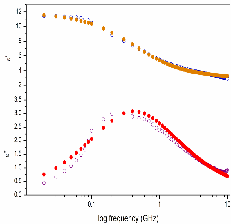
Fig. Complex Permittivity Spectra of PPG-425 at 300 K.
