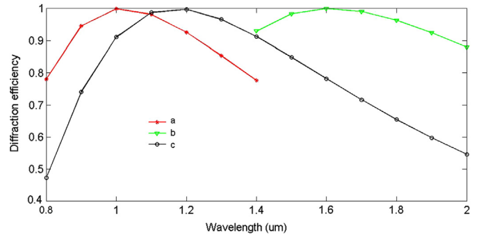
Fig. 3. Grating diffraction efficiency at different wavelengths: (a) band A, \lambda_B=1000 nm, i=12.6^\circ ; (b) band B, \lambda_B=1600 nm, i=6.7^\circ ; (c) bands A and B, \lambda_B=1150 nm, i=12.6^\circ ( i is the angle of incidence).
