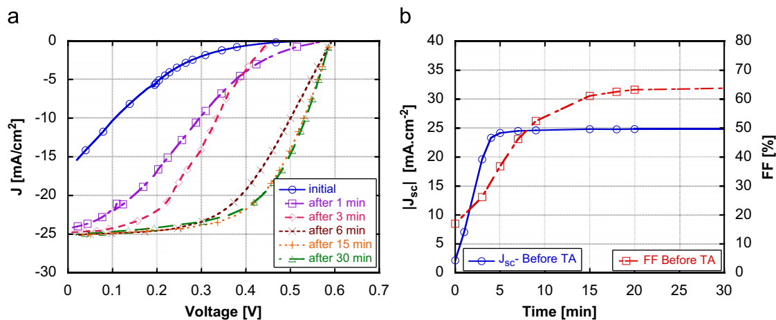
Fig. 1. AM 1.5 time dependent J ( V ) characteristics of a CIGSe/CBD-Zn(S,O,H)/rf-ZnMgO/ZnO:Al solar cell (a) and time variation of the corresponding short-circuit J_{sc} current density and fill factor (FF) (b), before thermal air annealing.
