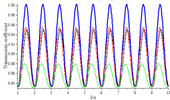
Transmission coefficient as a function of cavity length ( d_{LHM} = 450 nm).
