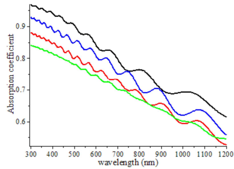
Absorption coefficient as a function of wavelength for pair metamaterial-dielectric multilayered structure ( d_{LHM} = 900 nm, d_{RHM} = 150 nm).
