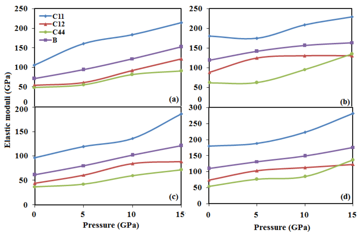
Variation of elastic moduli with pressure in B_2 phase for (a) ScZn, (b) TiZn, (c) YZn and (d) ZrZn
