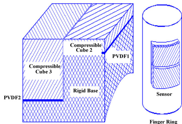
Fig. 1. Schematic of the designed probe with its major constituting parts.
