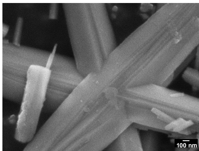
\alpha -Fe 2 O 3 doped with 10 mole % of Mn. The star branches consist of very thin lamellas.
