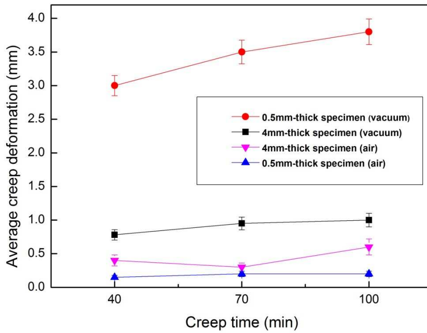
Creep deformation of specimens with different thicknesses under different atmospheres
