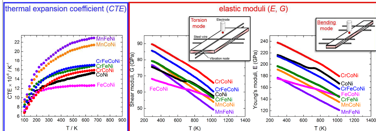
Temperature dependence of physical properties in medium entropy alloys
