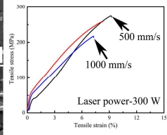
Stress-strain curve
