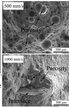
Fracture surface
