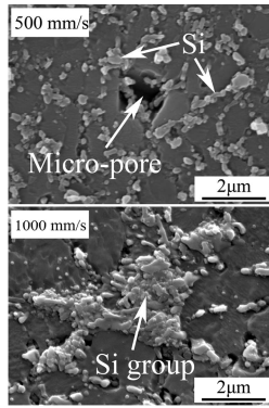
Microstructure
