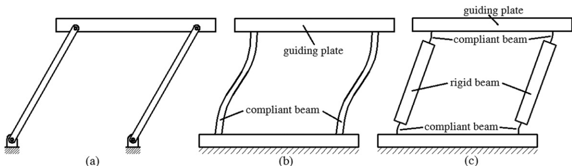
Fig. 1. Parallel-guiding mechanism: (a) RPGM; (b) distributed-CPGM; (c) lumped-CPGM.
