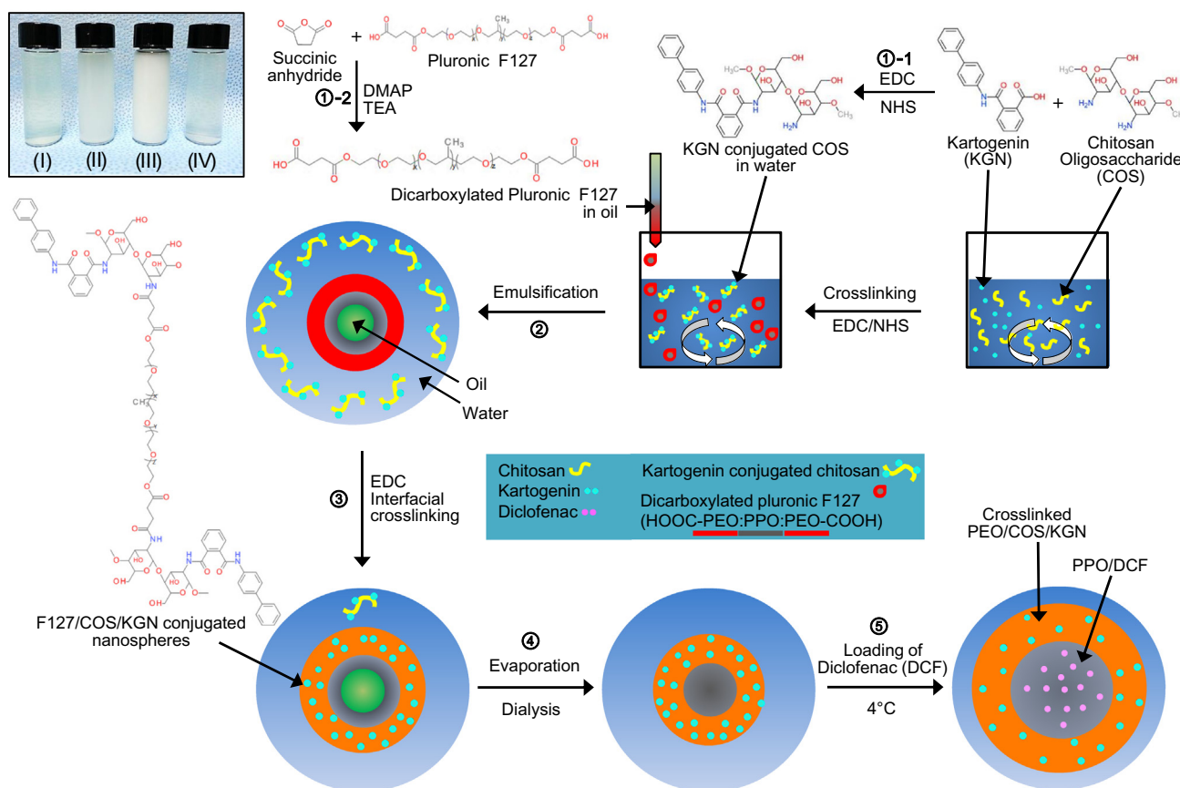
Fig. 1. Illustration of the procedure and chemistry to synthesize the F127/COS/KGN DCF nanospheres. The carboxyl group of KGN and the amine group of COS were covalently conjugated by EDC/NHS catalysis before nanosphere synthesis. Each hydroxyl end of pluronic F127 was grafted with a carboxyl group derived from succinic anhydride. Then, the remaining amine groups in the KGN-conjugated COS were covalently cross-linked with carboxyl groups of dicarboxylated pluronic F127 using an EDC catalyst during oil-in-water emulsification. DCF was loaded into the cross-linked F127/COS/KGN nanospheres by increased wall permeability due to the expansion after cold shock treatment. The pictures on upper left show the typical appearance of the KGN-conjugated COS (I), the oil-in-water emulsion of dicarboxylated pluronic F127 and KGN-conjugated COS before (II) and after (III) sonication, and after rotary evaporation to remove the organic phase (IV) [EDC, 1-ethyl-3-(3-dimethylaminopropyl)carbodiimide; NHS, N-hydroxysuccinimide; DMAP, 4-dimethylaminopyridine; TEA, triethylamine; COS, chitosan oligosaccharide; KGN, kartogenin; DCF, diclofenac; PEO, polyethylene oxide; PPO, polypropylene oxide].
