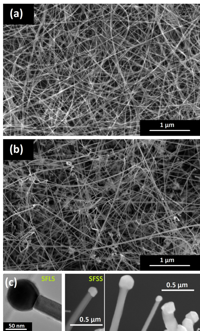
Fig. 1. The SEM images show Ge NWs grown in (a) supercritical toluene at 380 °C with a reactor pressure of 320 bar and (b) by low pressure CVD at 430 °C at 10^{-2} mbar using DPG as precursor. (c) Shows the observed shapes of the metal particle associated with a liquid growth promoter (SFLS mechanism; T > 340 °C) and solid seeds (SFSS mechanism; T = 250 °C).
