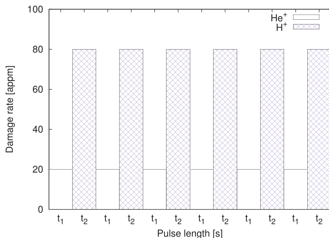
Fig. 1. Pulsed irradiation schematic of the second beamline in the dual-beam irradiation configuration. In the first beamline, \text{Fe}^{3+} emits at a steady dose rate of 1.6 \times 10^{-3} dpa/s same as in the steady triple-ion irradiation case.
