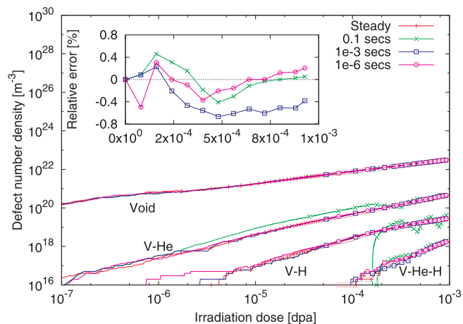
Fig. 2. Number density of various types of defects formed under pulsed dual-beam irradiations with short pulse-length compared to steady triple-beam irradiations. The inset shows relative differences in volume-swelling ratios obtained from these two irradiation methods.
