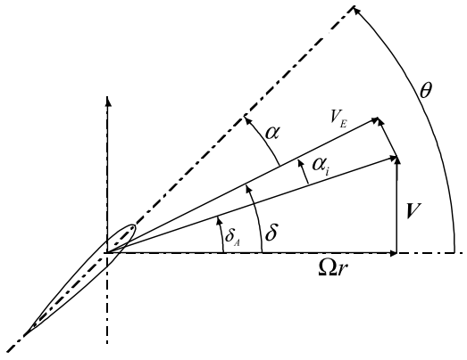
Fig. 1. Blade profile of radial position r .
