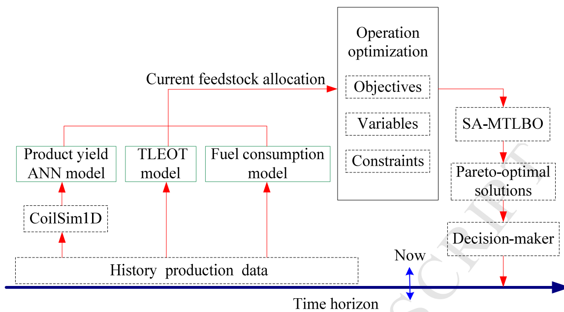
Multiobjective optimization for ethylene cracking furnace system
