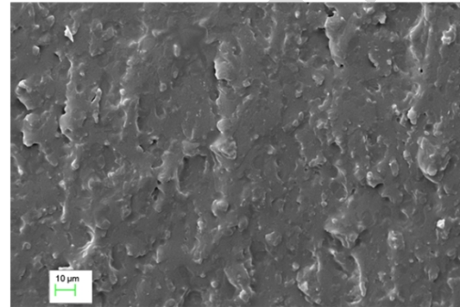
Compatibilized PLA-NR blend
