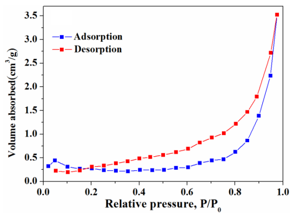
Graphical abstract: N 2 adsorption and desorption isotherms of activated sludge
