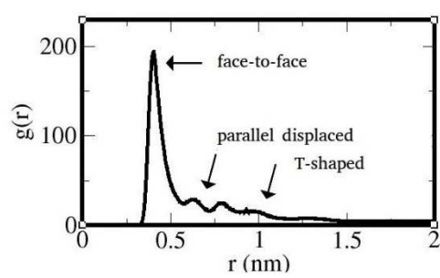
Radial distribution function of asphaltene
