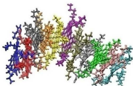
Asphaltene aggregate
