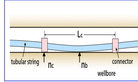
Local model
