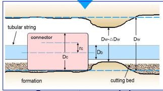
Connector model
