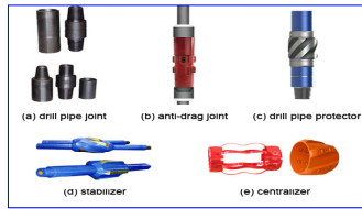
Common connectors
