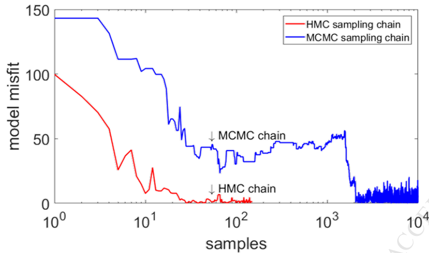
Faster converging speed by HMC
