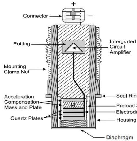
Fig.1 Fundamental diagram of dynamic pressure sensor
