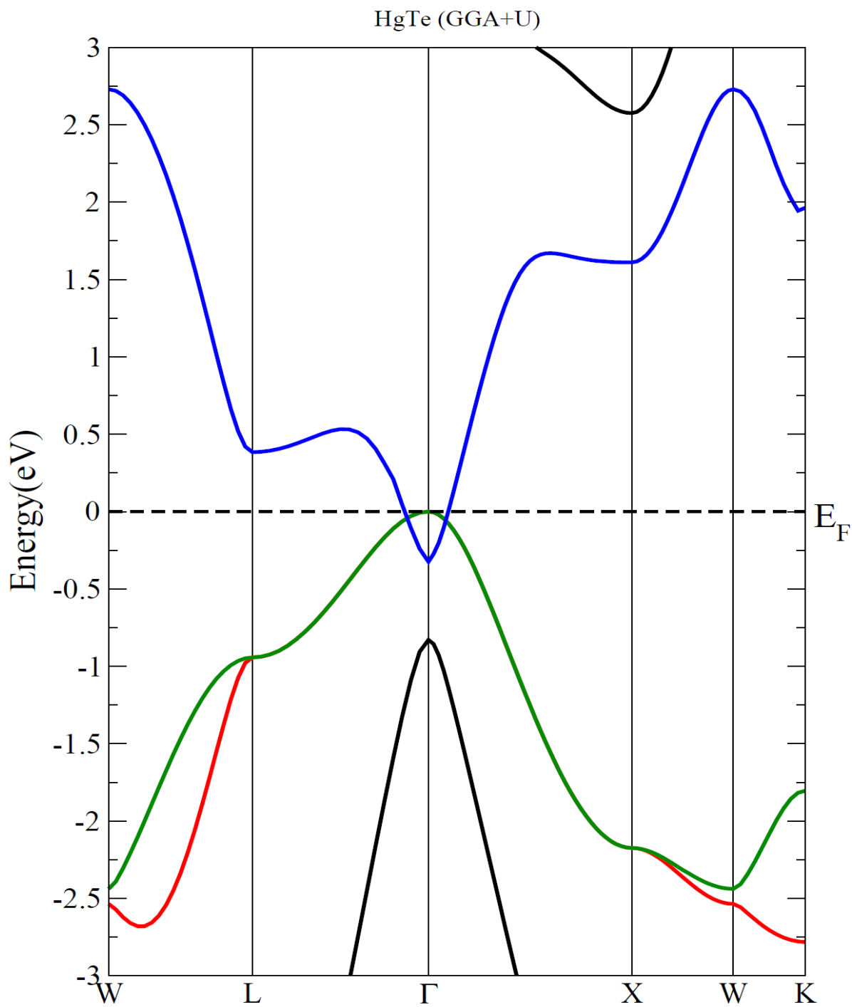
Electronic band structure of the HgTe using GGA+U functional
