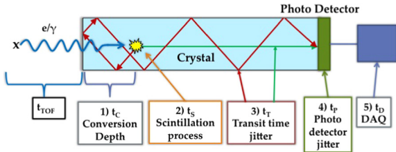
Fig. 1. Schematic showing various contributions to the resolution obtained when measuring time using crystal scintillation light [4].
