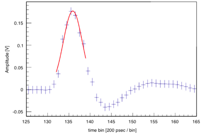
Fig. 4. Digitized pulse from the reference MCP-PMT, coarse-grained to show the pulse structure. A Gaussian fit to the pulse is used to extract a reference time stamp for the TOF measurement.
