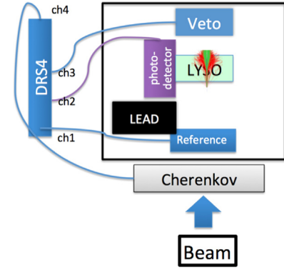
Fig. 3. Diagram of the setup used to measure electron time of flight with a 1.7 \times 1.7 \times 1.7 \text{ cm}^3 LYSO crystal interfaced with an MCP-PMT photodetector and read out using a DRS4 digitizer unit.
