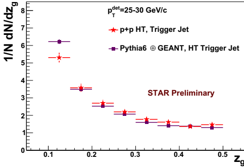
Figure 1: Trigger jets for p+p HT compared to PYTHIA predictions after simulation of the STAR detector. Independently binned in one example p_T^{\text{det}} bin at detector level. Error bars are statistical only.
