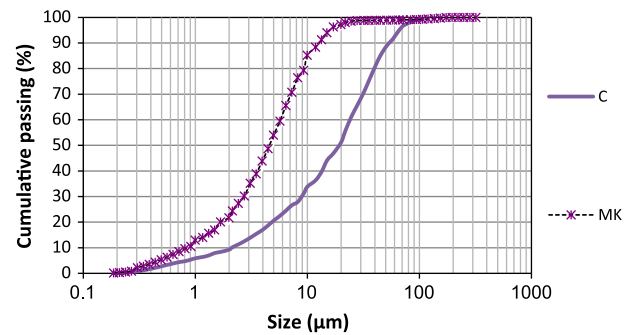
Fig. 1. Particle size distribution of powders.
