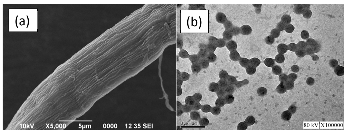
(a) SEM image of cellulose fibers facial cotton and (b) TEM micrograph of cellulose nanoparticles prepared from 0.01 w/v % of cellulose solution
