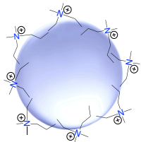
DMAB-stabilized nanoparticles
