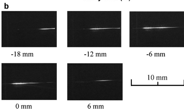
Fig. 2. (a) Time-resolved two-color OKS signals, and (b) recorded images of the formed filament in the sample, when the 10-mm-thick sample was fixed at different positions. The pump power was fixed at 3 mW.
