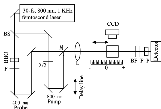
Fig. 1. Schematic diagram of the experimental setup. BS: beam splitter, F: filter, M: dielectric mirror, L: convex lens, BF: bandpass filter, P: polarizer.
