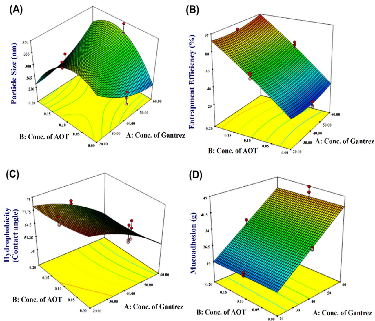
Fig. 1. Contour plots showing the effects of Concentration of Gantrez AN-119 (%w/w of total Gantrez and Glyceryl monostearate amount) and concentration of Docusate sodium, AOT (% w/v of aqueous phase) on (A) the average particle size, (B) % entrapment efficiency (%EE), (C) hydrophobicity and (D) mucoadhesion of RIF nanoparticles.
