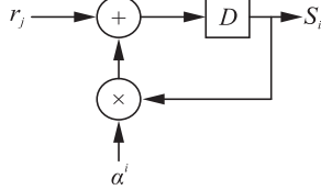
Fig. 1 Basic syndrome calculator cell
