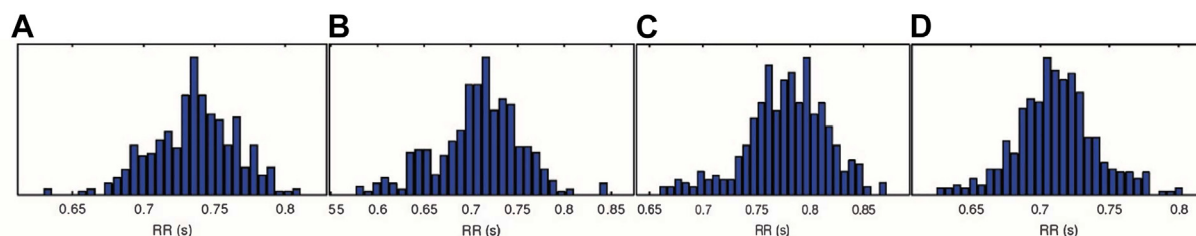
Figure 1 Time-domain results—RR interval distributions: (A) concussion at rest, (B) concussion postexercise, (C) recovered at rest, and (D) recovered postexercise.
