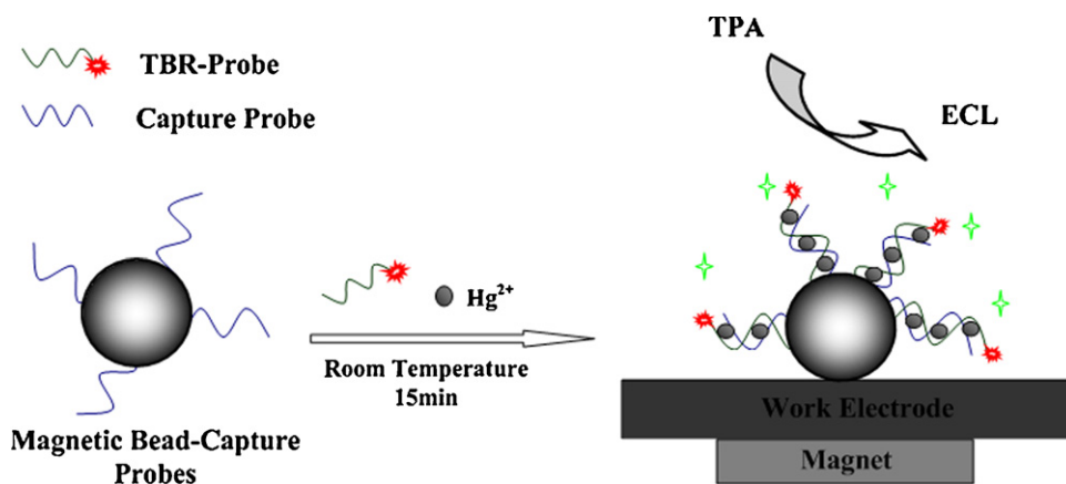
Scheme 1. Schematic illustration of the magnetic beads-based ECL assay for detection of \text{Hg}^{2+} .
