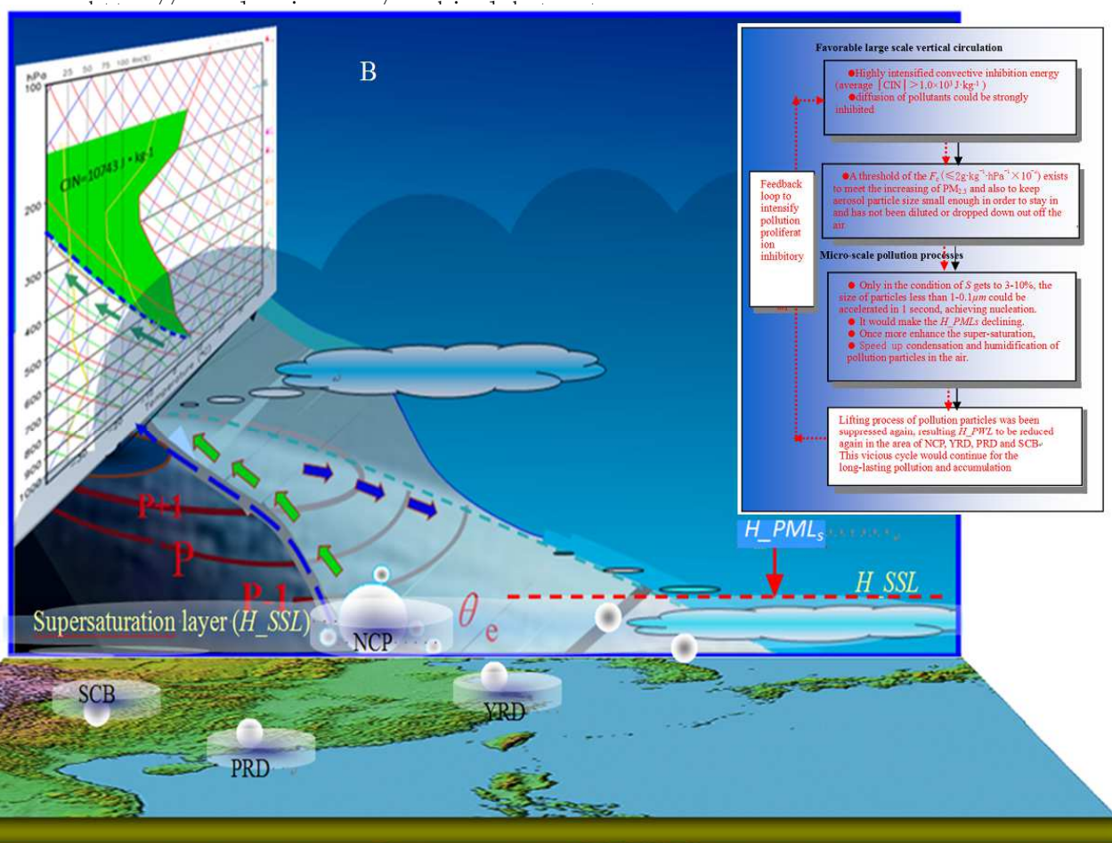
Fig.6. Schematic diagram of 3-D model for low-level super-saturation layer ( H_{SSL} ) and pollution mixing layer ( H_{PMLs} ) in the pollution hotspots (NCP, YRD and PRD and SCB) in China. Light blue scarping down to the bottom of the vertical plane (B) is iso- \theta_e surface for air adiabatic uplift; on the upper left corner of B-plane is the tephigram.
