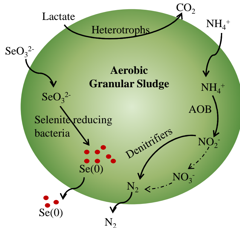
Simultaneous COD, nitrogen and selenite removal by aerobic granular sludge
