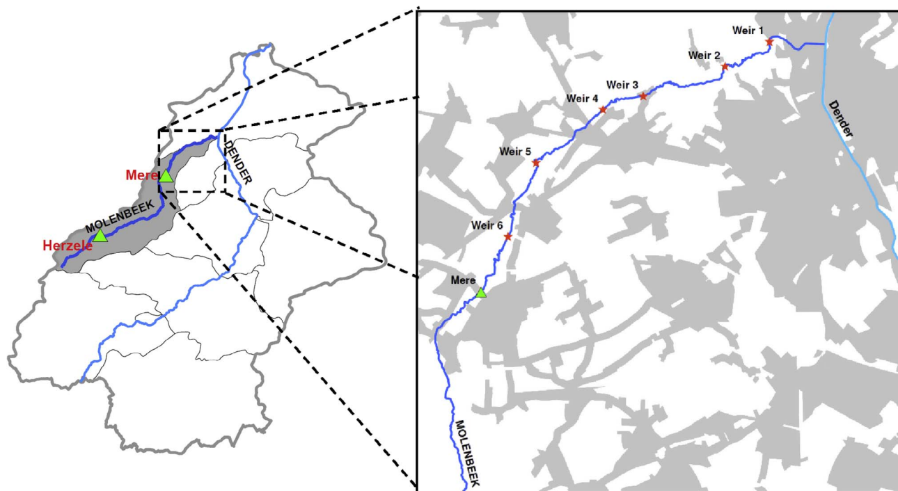
Fig. 1. Overview of the river Molenbeek catchment within the river Dender basin (left). Zoomed view on the measurement locations (right). Green triangles depict limnigraphic stations, red stars adjustable control structures and grey zones the urbanized regions. (For interpretation of the references to colour in this figure legend, the reader is referred to the web version of this article.)
