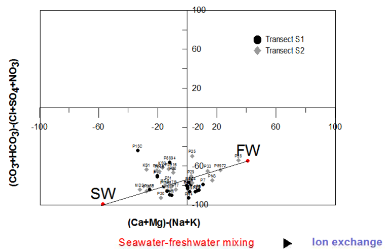
Seawater intrusion in transect S1
