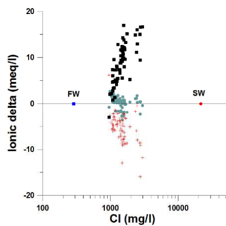
Seawater intrusion in transect S1
