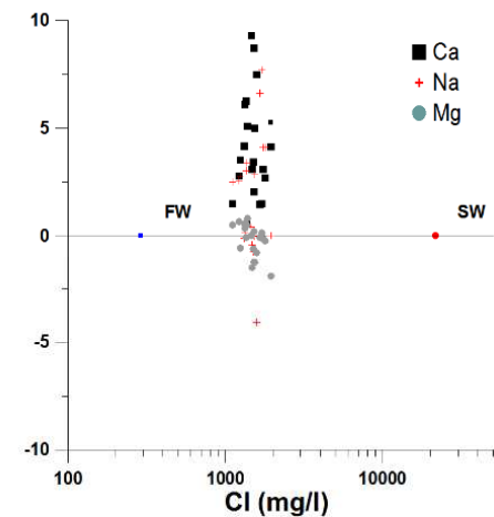
freshwater flushing in transect S2
