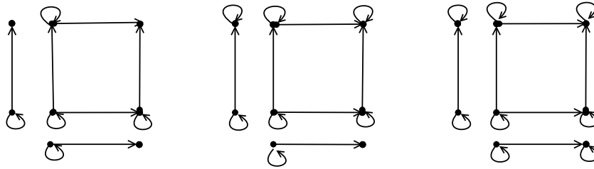
Fig. 1. Cartesian products of graphs with loops.
