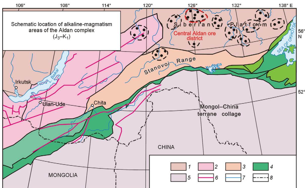
Fig. 1. Schematic geologic location of the Central Aldan ore district in the area of the Aldan alkaline complex (after A.S. Borisenko and G.S. Fedoseev). 1, Siberian Platform; 2, Baikalsk-Patom belt; 3, Stanovoi area; 4, Mongol-Okhotsk belt; 5, Mongol-China terrane collage; 6, faults; 7, water reservoirs; 8, state borders. Red dashed contour marks the Central Aldan ore district, and black contours show local areas of the Late Mesozoic alkaline magmatism.
