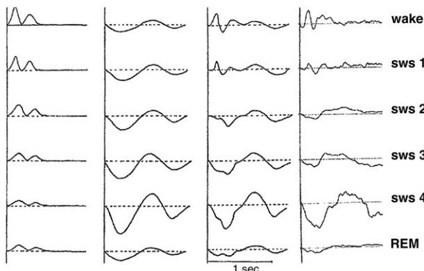
Fig. 1. In the most-right panel the grand averages of auditory evoked potentials of sleep–wake states (wake, SWS 1–SWS 4, REM) derived from position Cz are shown (voltage on the Y-axis is given in arbitrary units [negativity upward] and the time scale is indicated). In the most-left panel modelling according to the factor 'sensory gating' is presented, while in the middle-left panel modelling according to the factor 'neuronal firing mode' is indicated. Both modelling factors are described and discussed in the text. In the middle-right panel the results of the modelling with these two factors are combined, simply by addition. Note the remarkable resemblance between the constructed evoked potentials in this middle-right panel with the original recordings in the most-right panel.
