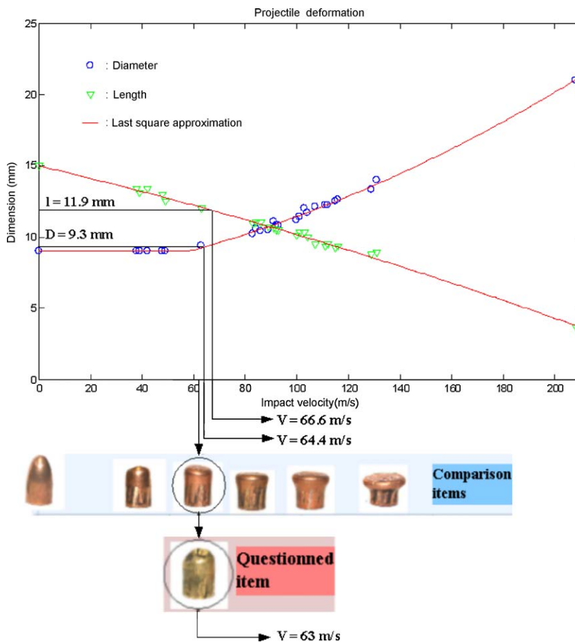
Fig. 1. Dimension of the bullet (length and diameter) for various impact bullet velocities.
