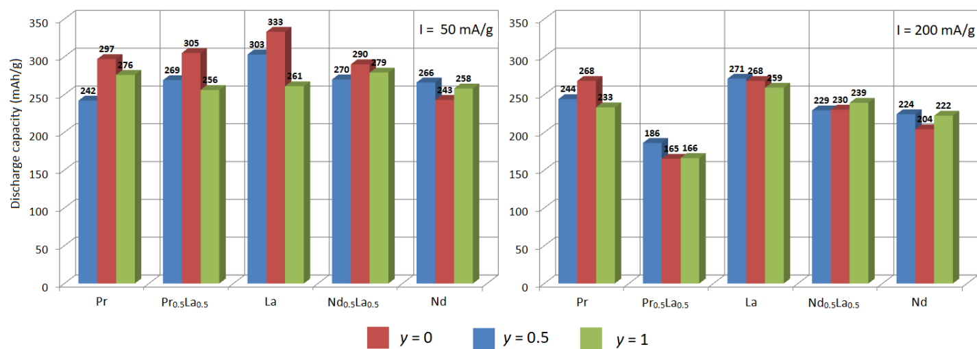
Discharge capacities of the R_{1-x}R'_x\text{MgNi}_{4-y}\text{Co}_y alloys
