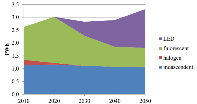
Fig. 5. Electricity demand for lighting by lamp technology.
