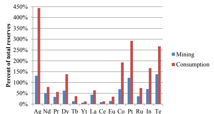
Fig. 6. Metals cumulative need for clean energy technologies until 2050 in relation to global mineral reserves.
